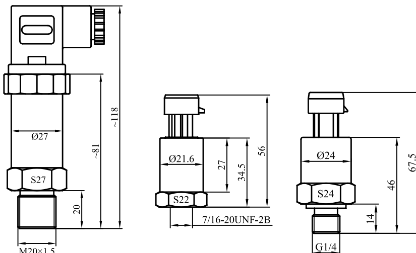
Dimension in:mm
